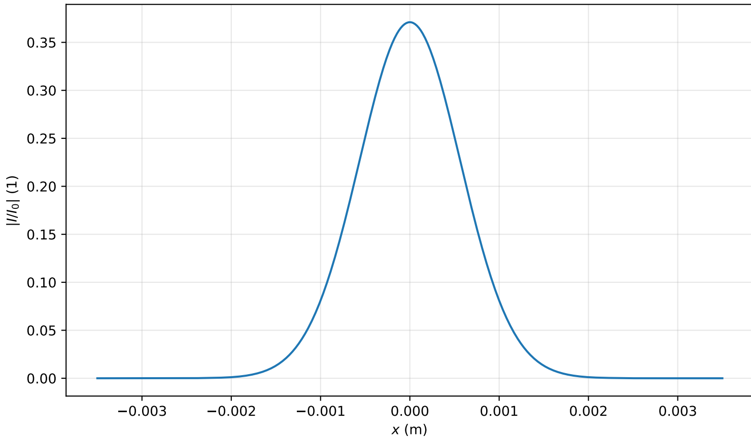
Intensity profile I(x, y = 0, z = 2.786m)/I_0 , P_{in}=0.1P_{cr} , artificial time
